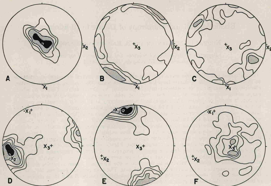
Fig. 1. Orientation diagrams for 200 grains of olivine in dunite A (A-C) and dunite B (D-F): (A) a axes, contours 10%, 5%, 3%, and 1% per 1% area; (B) b axes and (C) c axes, contours 5%, 3%, and 1% per 1% area; (D) b axes and (E) a axes, contours 10%, 7%, 5%, 3%, and 1% per 1% area; (F) c axes, contours 7%, 5%, 3%, and 1% per 1% area.
